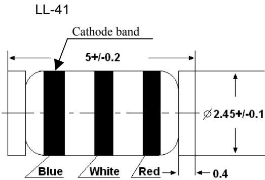
Glass case MELF Dimensions in mm
