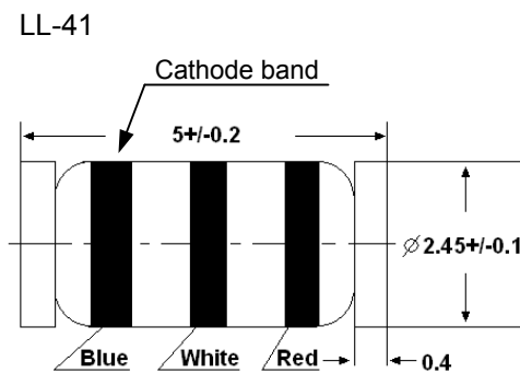
Glass case MELF Dimensions in mm
