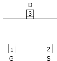
SOT - 23 -3 Top View
