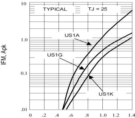
Fig. 2-FORWARD CHARACTERISTICS
