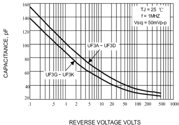
Fig. 6-TYPICAL JUNCTION CAPACITANCE
