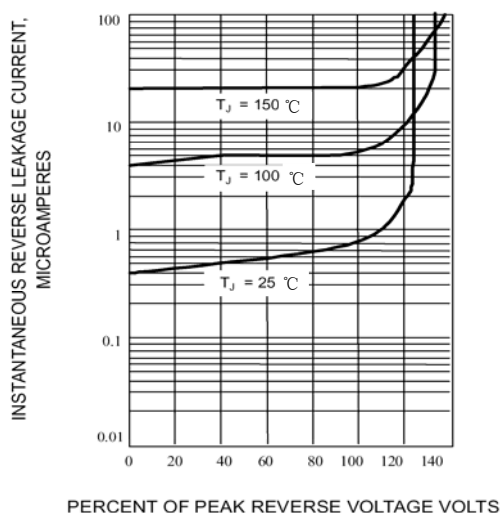
Fig. 3-TYPICAL REVERSE CHARACTERISTICS
