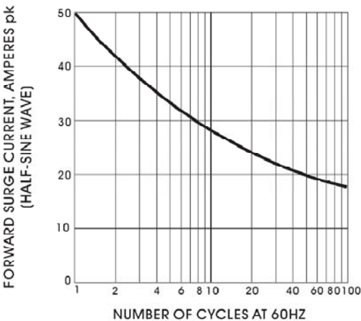
Fig.3-MAXIMUM OVERLOAD SURGE-CURRENT
