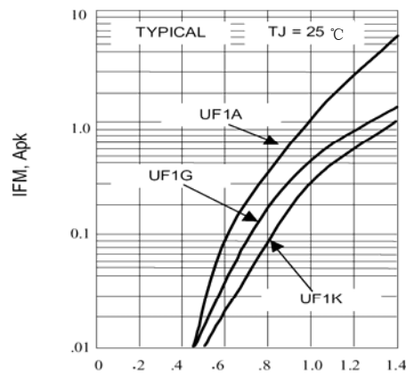
Fig. 2-FORWARD CHARACTERISTICS
