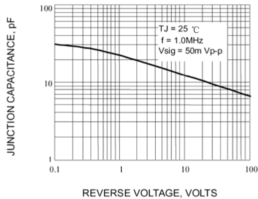
Fig. 4-TYPICAL JUNCTION CAPACITANCE
