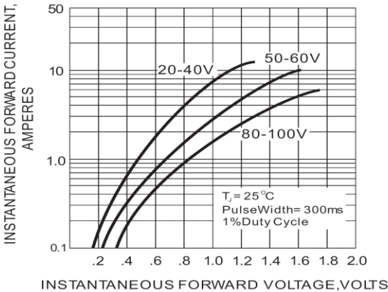
Fig.2-TYPICAL INSTANTANEOUS FORWARD CHARACTERISTIC
