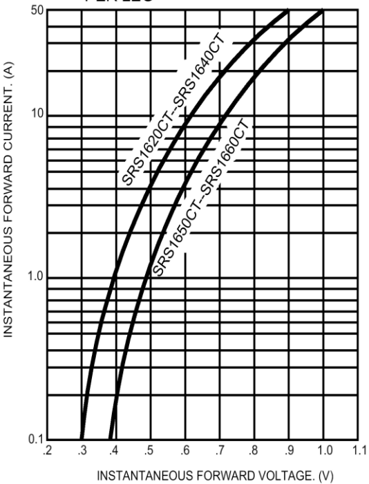
FIG.4- TYPICAL FORWARD CHARACTERISTICS PER LEG
