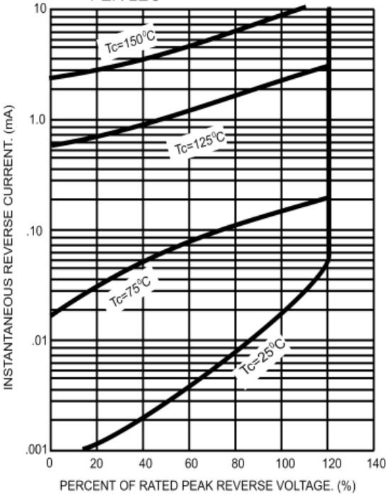
FIG.2- TYPICAL REVERSE CHARACTERISTICS PER LEG
