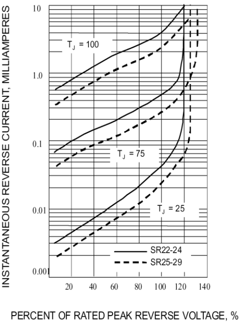
Fig. 3-TYPICAL REVERSE CHARACTERISTICS
