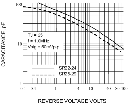
Fig. 4-TYPICAL JUNCTION CAPACITANCE
