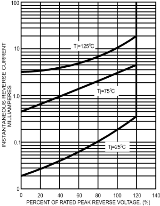
FIG.3- TYPICAL REVERSE CHARACTERISTICS PER LEG
