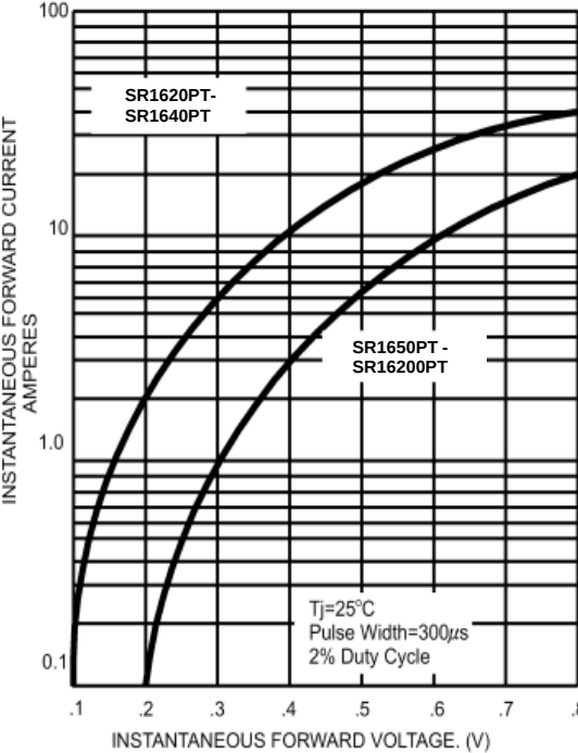
FIG.4- TYPICAL INSTANTANEOUS FORWARD CHARACTERISTICS PER LEG
