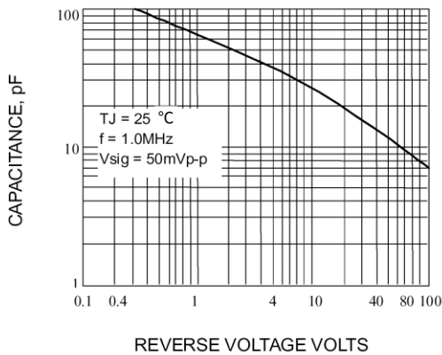
Fig. 4-TYPICAL JUNCTION CAPACITANCE
