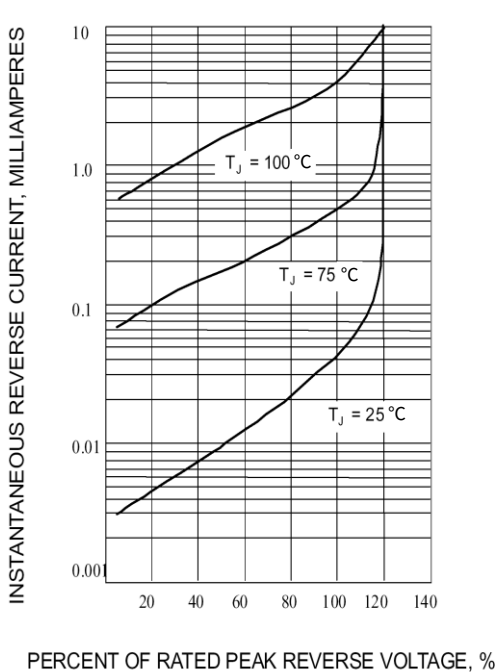
Fig. 3-TYPICAL REVERSE CHARACTERISTICS
