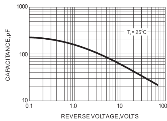
Fig.3-TYPICAL JUNCTION CAPACITANCE
