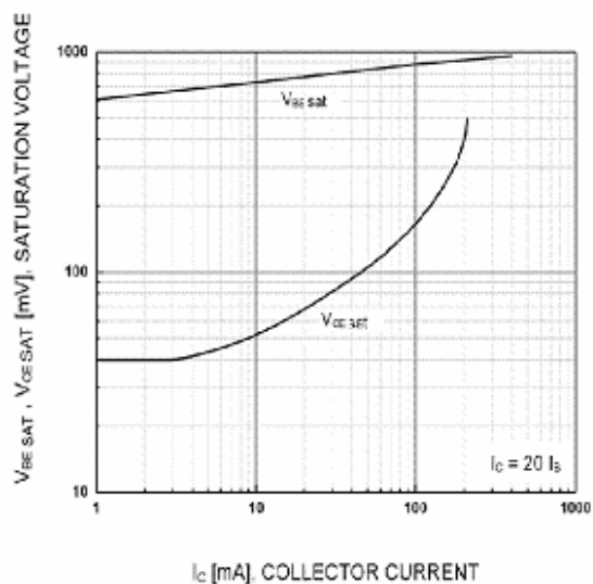
Base-Emitter Saturation Voltage Collector-Emmitter Saturation Voltage
