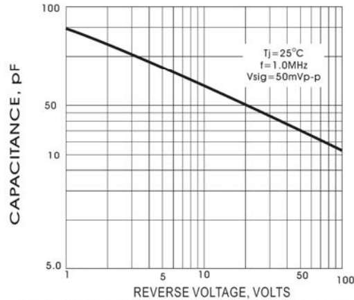
Fig. 5- TYPICL JUNCTION CAPACITANCE PER ELEMENT
