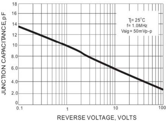
Fig. 5-TYPICAL JUNCTION CAPACITANCE
