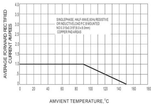
Fig. 2-MAXIMUM AVERAGE FORWARD CURRENT RATING
