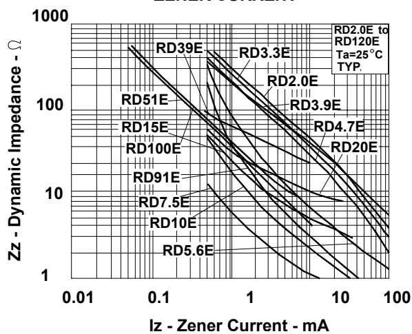
DYNAMIC IMPEDANCE vs. ZENER CURRENT
