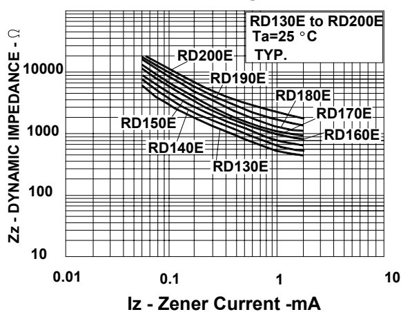
DYNAMIC IMPEDANCE vs. ZENER CURRENT
