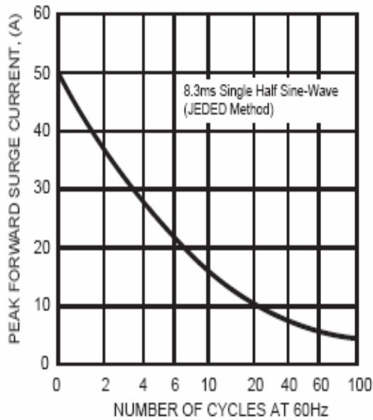
FIG. 1 - MAXIMUM NON-REPETITIVE FORWARD SURGE CURRENT
