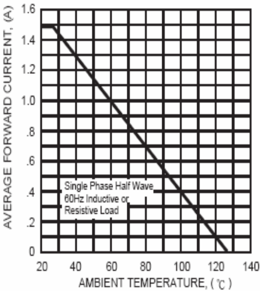
FIG. 2 - TYPICAL FORWARD CURRENT DERATING CURVE
