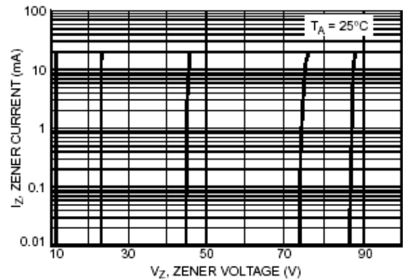
Figure 10. Zener Voltage versus Zener Current
