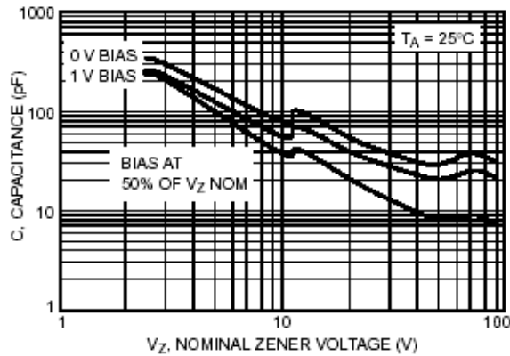
Figure 7. Typical Capacitance
