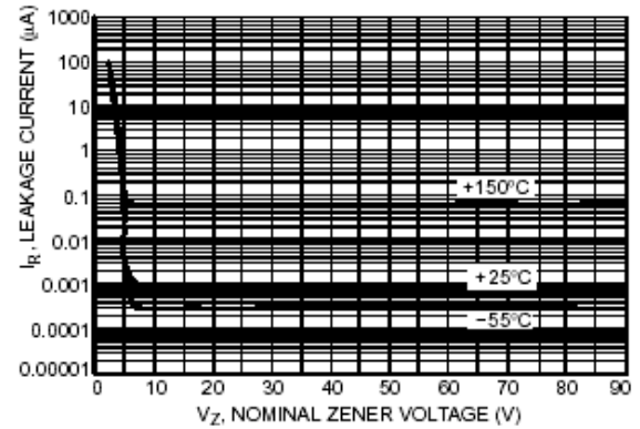
Figure 8. Typical Leakage Current
