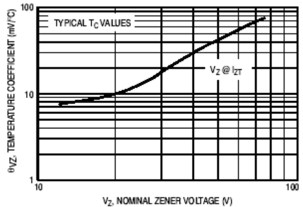
Figure 2. Temperature Coefficients (Temperature Range -55°C to +150°C)
