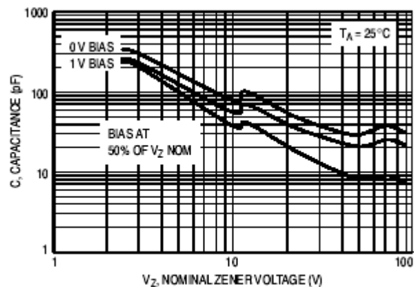
Figure 7. Typical Capacitance
