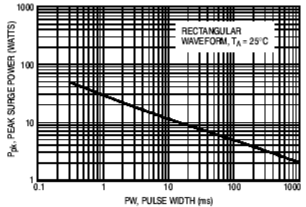
Figure 4. Maximum Nonrepetitive Surge Power
