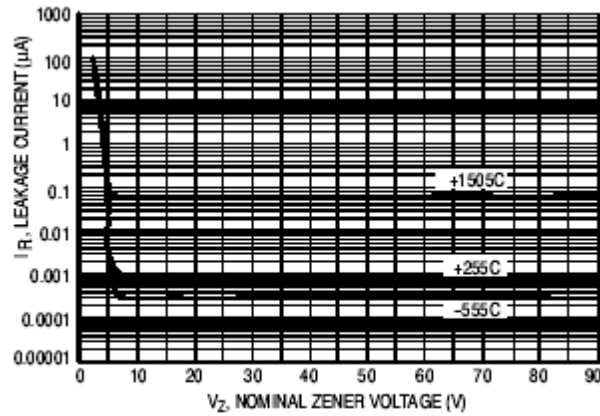
Figure 8. Typical Leakage Current
