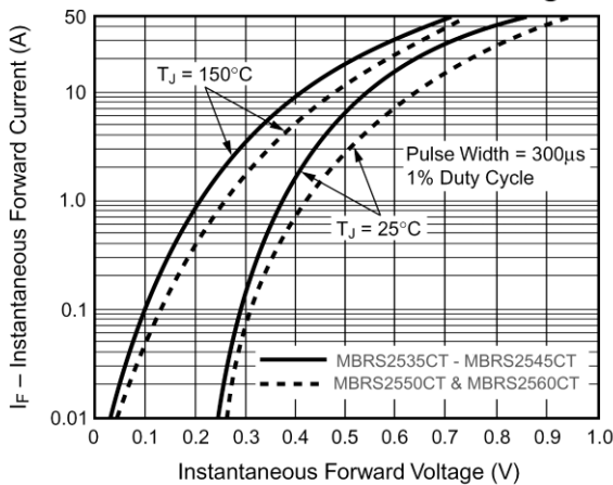
Typical Instantaneous Forward Characteristics Per Leg
