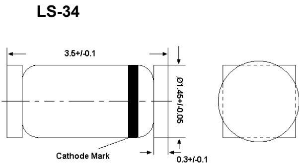
Glass case MiniMELF
