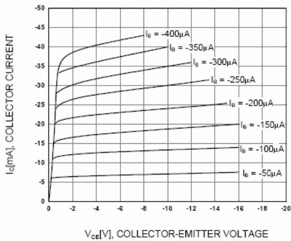
Figure 1. Static Characteristic
