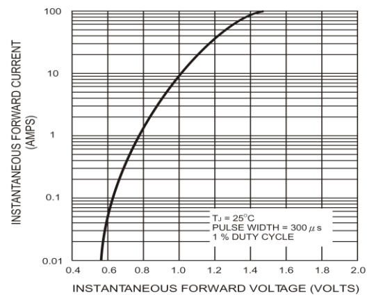
Figure 2. Typical Instantaneous Forward Characteristics Per Bridge Element
