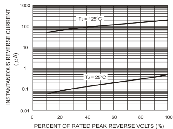
Figure 4. Typical Reverse Leakage Characteristics Per Bridge Element
