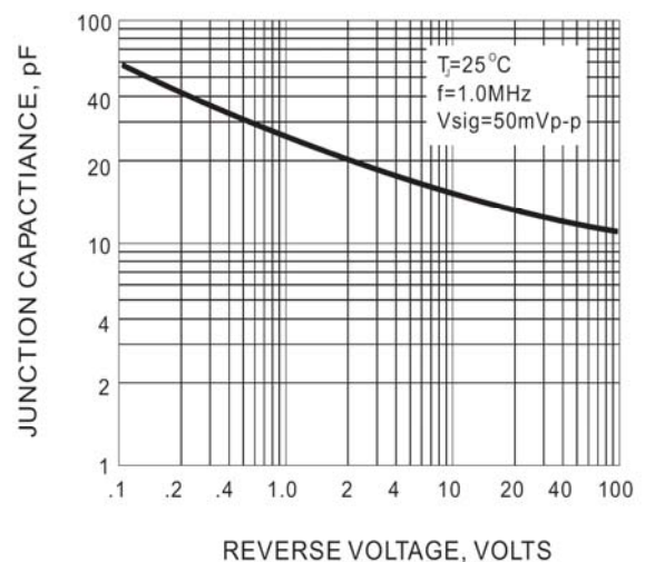
Fig.6- TYPICAL JUNCTION CAPACITANC
