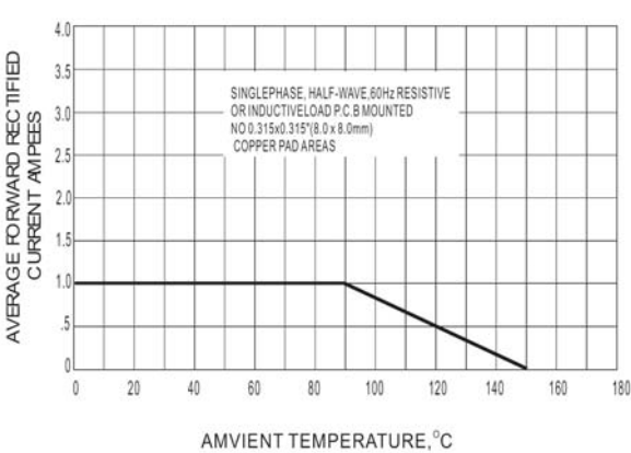
Fig. 2-MAXIMU AVERAGE FORWARD CURRENT RATING
