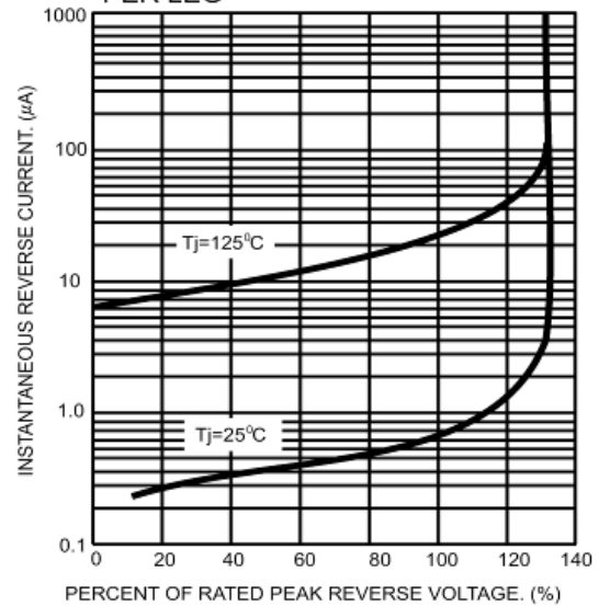
FIG.5- TYPICAL REVERSE CHARACTERISTICS PER LEG
