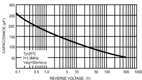
FIG.4- TYPICAL JUNCTION CAPACITANCE PER LEG
