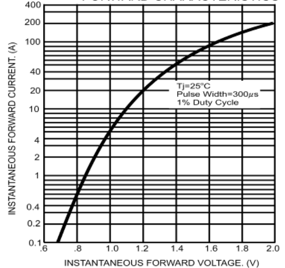
FIG.5- TYPICAL INSTANTANEOUS FORWARD CHARACTERISTICS
