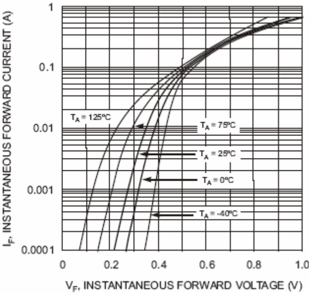
Fig. 2 Forward Characteristics
