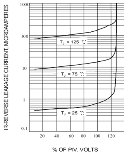
Fig. 3-TYPICAL REVERSE CHARACTERISTICS
