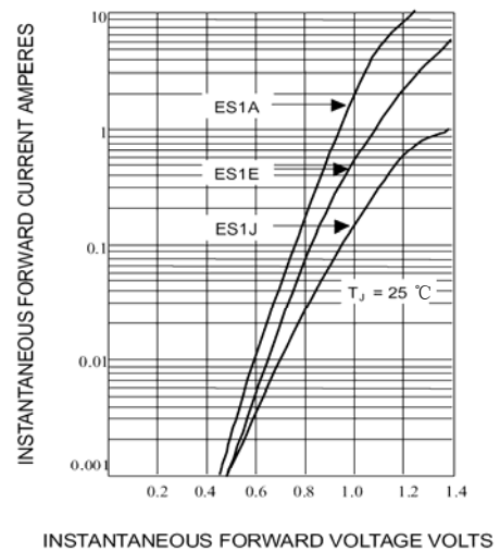
Fig. 4-TYPICAL FORWARD CHARACTERISTICS
