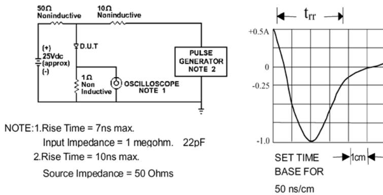
Fig. 1-REVERSE RECOVERY TIME CHARACTERISTIC AND TEST CIRCUIT DIAGRAM
