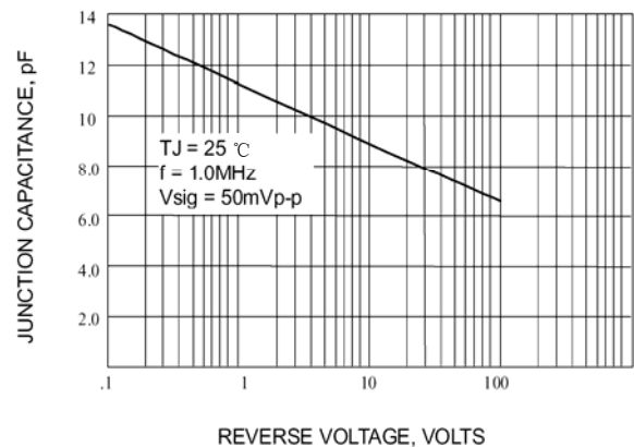
Fig. 6-TYPICAL JUNCTION CAPACITANCE
