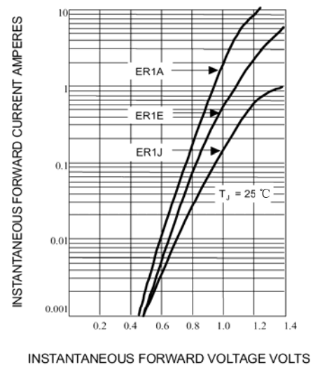
Fig. 4-TYPICAL FORWARD CHARACTERISTICS
