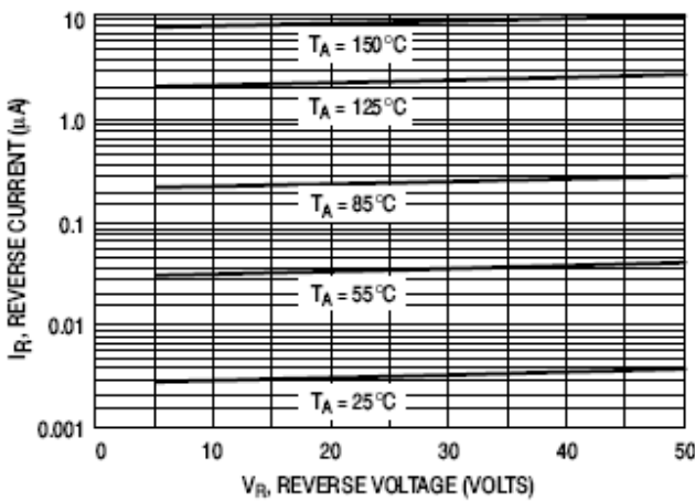
Figure 2. Leakage Current
