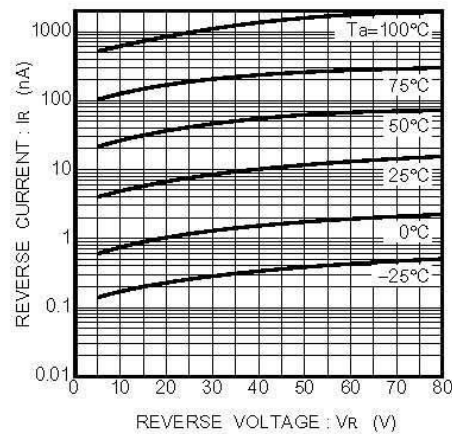
Reverse characteristics
