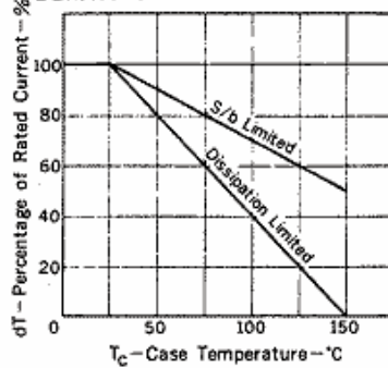
DERATING CURVES FOR ALL TYPES
