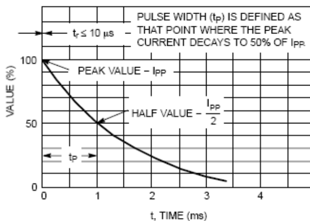
Figure 2. 10 x 1000 \mu\text{s} Pulse Waveform
