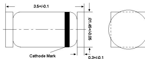
Glass case MiniMELF Dimensions in mm
