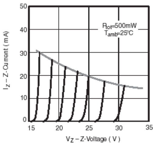
Figure 8. Z-Current vs. Z-Voltage
