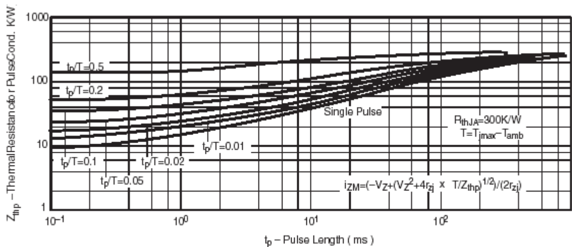
Figure 10. Thermal Response
