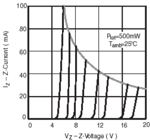
Figure 7. Z-Current vs. Z-Voltage
