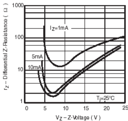
Figure 9. Differential Z-Resistance vs. Z-Voltage
