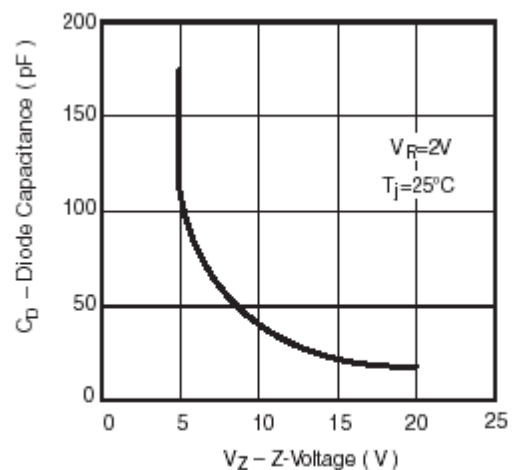
Figure 5. Diode Capacitance vs. Z-Voltage
