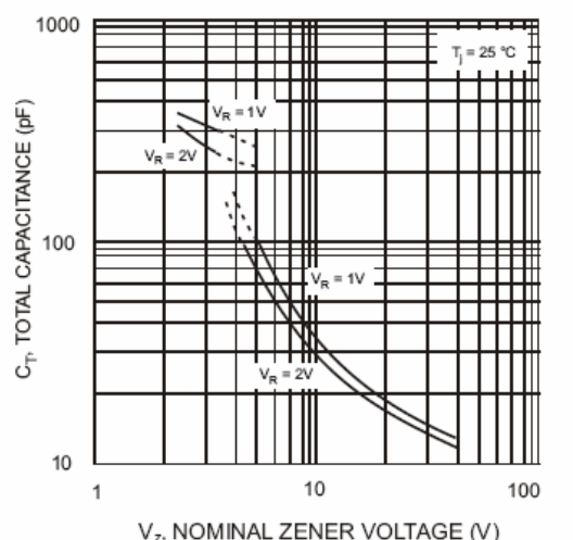
Fig. 5 Total Capacitance vs. Nominal Zener Voltage
