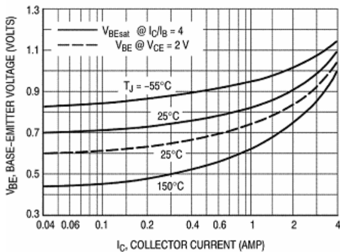
Base-Emitter Voltage
