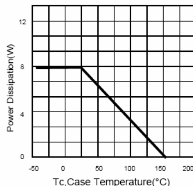
Fig.3 Power Derating
