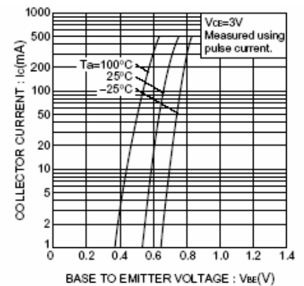
Fig.3 Grounded emitter propagation characteristics
