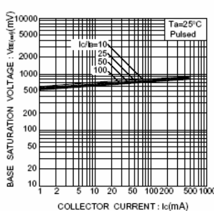
Fig.8 Base-emitter saturation voltage vs. collector current(I)
