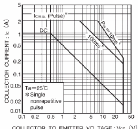
Fig.9 Safe operating area (2SD1664)
