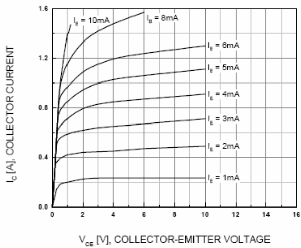
Figure 1. Static Characteristics
