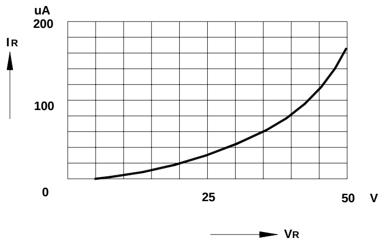
Reverse Characteristics
