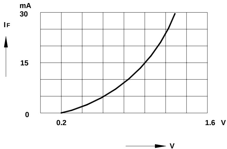
Forward Characteristics
