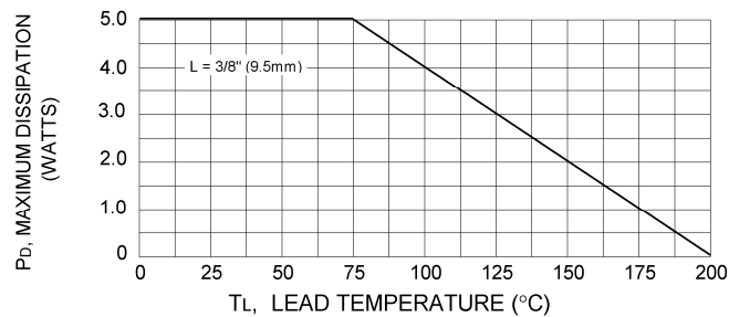
Fig. 1 POWER TEMPERATURE DERATING CURVE
