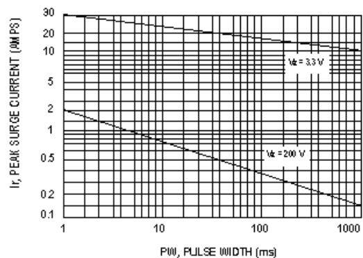
Fig. 4 Peak Surg Current versus Pulse Width
