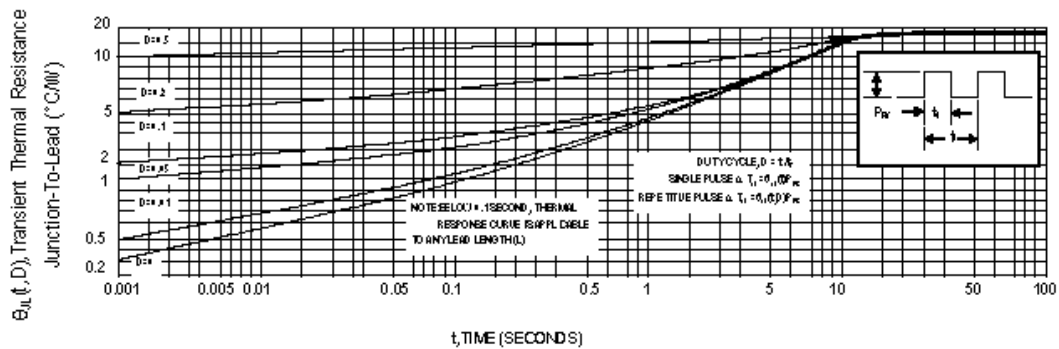
Fig 2. Typical Thermal Response L, Lead Length = 3/8 Inch
